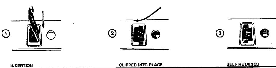
DIAGRAM 2 - INSERTION OF CAGE NUTS
